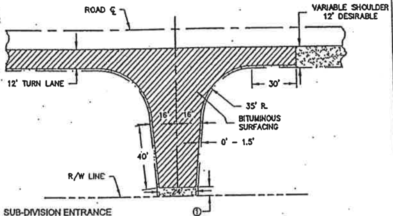
SUB-DIVISION ENTRANCE NO SCALE
