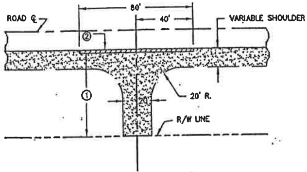
FIELD ENTRANCE NO SCALE
