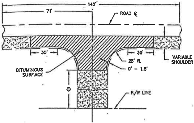
COMMERCIAL - INDUSTRIAL - FARM ENTRANCES NO SCALE
