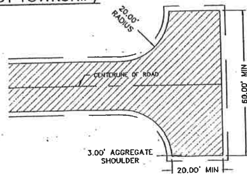
STANDARD T-TYPE TURNING AREA
