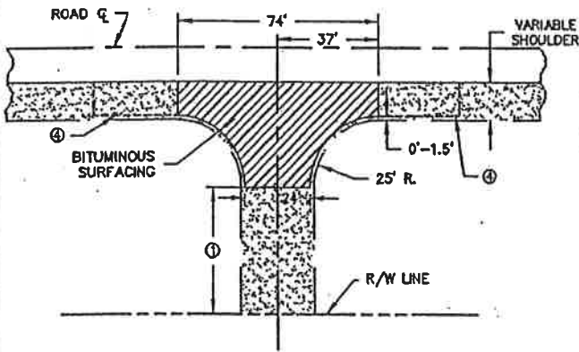
RURAL RESIDENTIAL ENTRANCE NO SCALE
