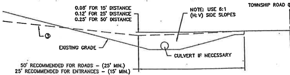
CROSS SECTION NO SCALE
