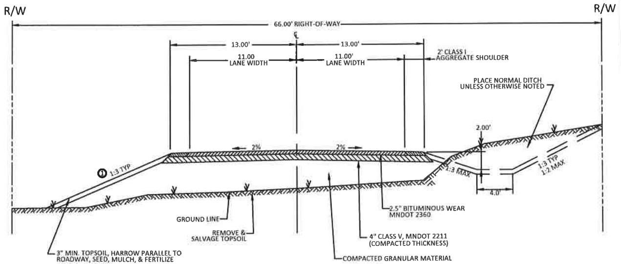
MINOR COLLECTOR TYPICAL SECTION SCALE: NONE
