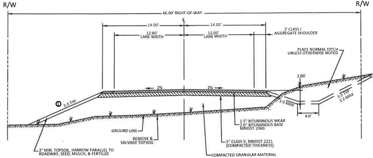
MAJOR COLLECTOR TYPICAL SECTION SCALE: NONE
