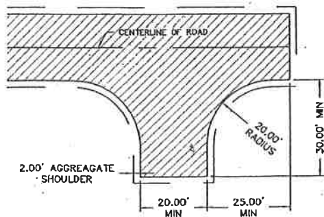
BRANCH TYPE TURNING AREA
